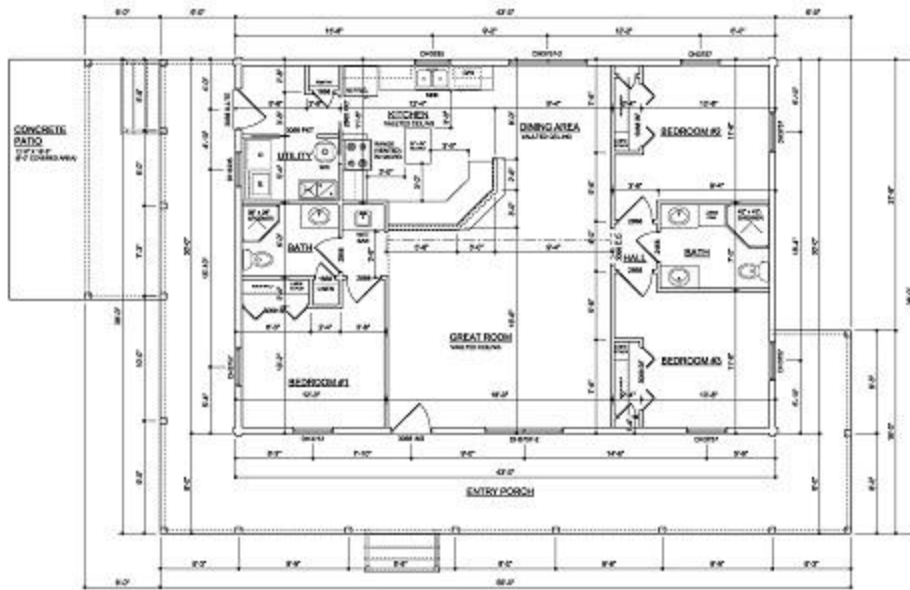
FLOOR PLAN SCALE 1/8" = 1'-0"
